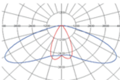
Luminance Intensity Distribution
